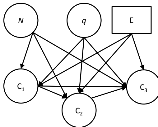
Figure 1.1. Directed acyclic graph of the removal fishing problem. Round shapes denote uncertain quantities, boxes represent known or controllable quantities, and arrows denote the direction of the causal relationship.
