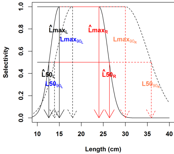
Figure 2. An example of a double normal selectivity curve where the most likely (modal) length at 50% selectivity on the left-hand side ( \hat{L}_{50_L} ) is 12.5 cm and on the right-hand side ( \hat{L}_{50_R} ) is 26.4 cm. The most likely range for selectivity equal to 1 is between 15 cm ( \hat{L}_{max_L} ) and 24 cm ( \hat{L}_{max_R} ). The 0.90 quantile for L_{50_L} ( L_{50_{90_L}} ) is 14 cm, and the 0.90 quantile for L_{50_R} ( L_{50_{90_R}} ) is 36 cm.
